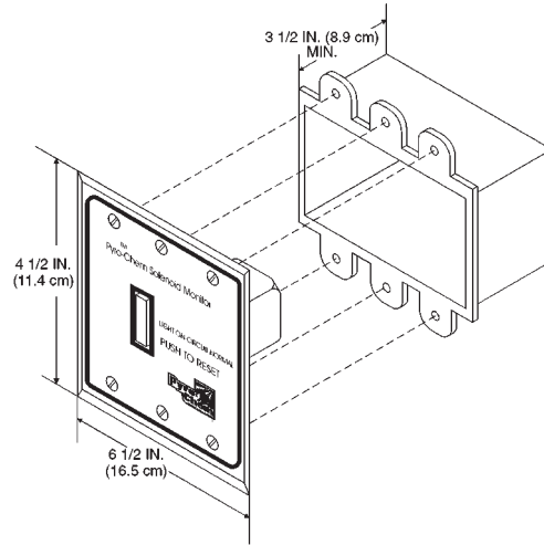
Figure 4-14. Solenoid Monitor Installation. 002881PC
