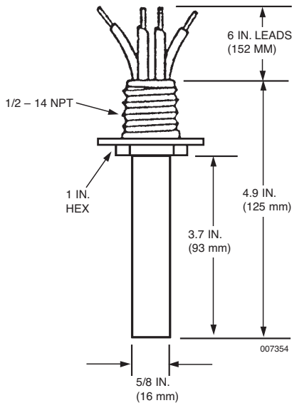
Figure 2-12a. Thermal Detector. 007354
