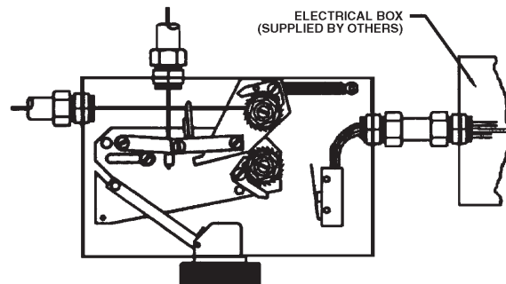
Figure 4-21. Micro Switch Installation in Model MCH3/NMCH3 Control Head. 002889PC
